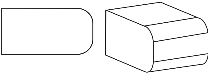
ROUND OVER TOP & BOTTOM (1/2" radius)
